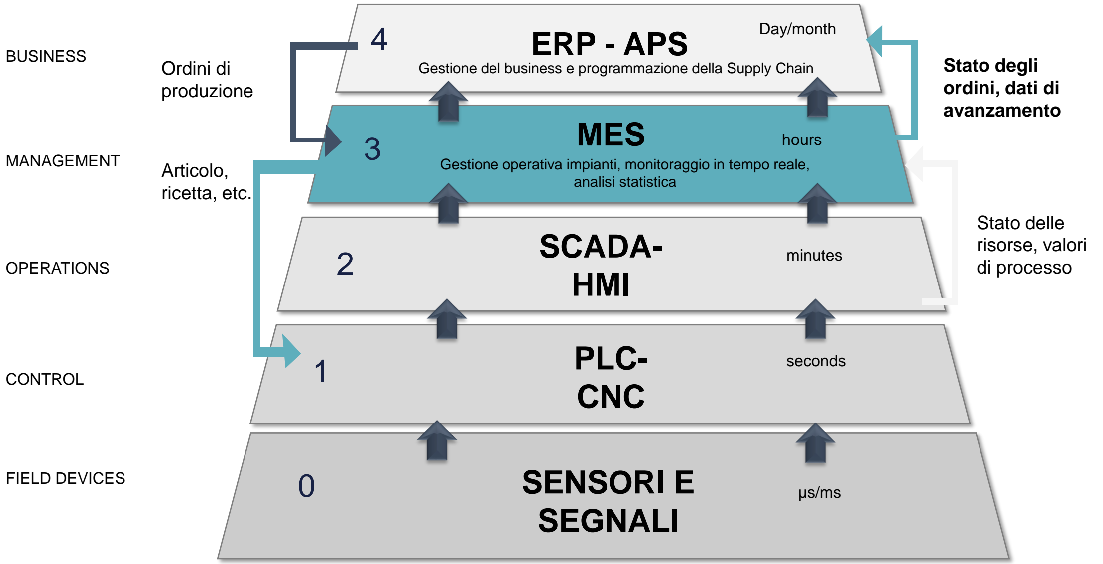
ISA 95 automation pyramid
